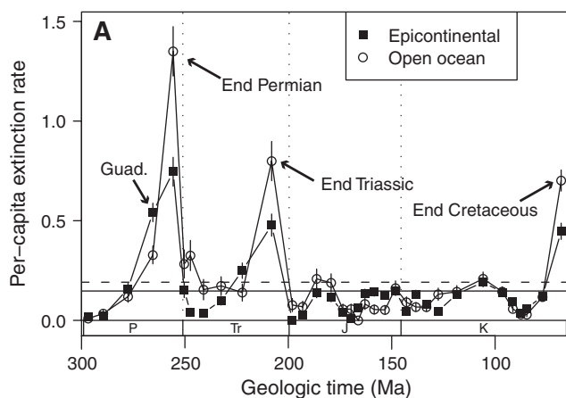
Fig. 1. Stage-by-stage depictions of extinction rates (A), origination rates (B), and mean geographic ranges (C) for genera in open-ocean-facing settings (1489 total genera) and epicontinental seas (1929 total genera) for the Permian through Cretaceous periods. Error bars are standard errors based on bootstrap resampling of genus stratigraphic ranges for evolutionary rates and of genus occurrences within stages for geographic ranges (500 replicates). For depictions of evolutionary rates, long-term means are illustrated with the horizontal lines: solid for epicontinental seas and dashed for open-ocean-facing settings. Abbreviations are as follows: P, Permian; Tr, Triassic; J, Jurassic; K, Cretaceous; and Ma, million years ago. (A) Extinction rates in both settings do not differ appreciably except during major mass extinctions in the Late Permian (Guadalupian and end-Permian), end-Triassic, and end-Cretaceous. In all of these cases except the Guadalupian, rates for open-ocean-facing settings significantly exceeded those for epicontinental seas. (B) Origination rates were generally more volatile than extinction rates, with no consistent difference between the two regimes until the Kimmeridgian; thereafter, open-ocean rates exceeded those for epicontinental seas in nearly every stage. (C) Mean geographic ranges of genera, which are based on convex-hull area scaled to the maximum possible (15), exhibit a volatile pattern through the study interval but nevertheless depict a significant downward trend for open-ocean-facing settings through the Late Jurassic.
