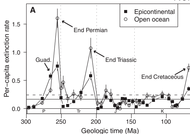
Fig. 2. Stage-by-stage depictions of extinction rates (A) and origination rates (B) for non-bivalve genera in open-ocean-facing settings (1088 total genera) and epicontinental seas (1617 total genera) for the Permian through Cretaceous periods. Salient features observed in Fig. 1, including
